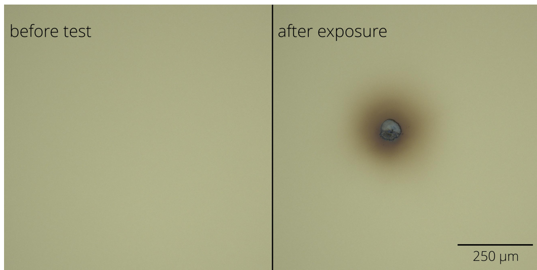
Figure 5. Typical damage morphology: fluence 23.8 \text{ J/cm}^2 , damage after 154 pulse(s).
