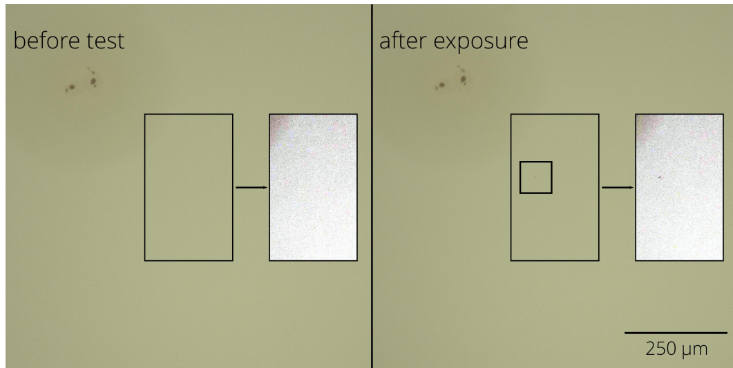
Figure 4. Typical damage morphology: fluence 16.0 \text{ J/cm}^2 , damage after 1000 pulse(s). High contrast image.
